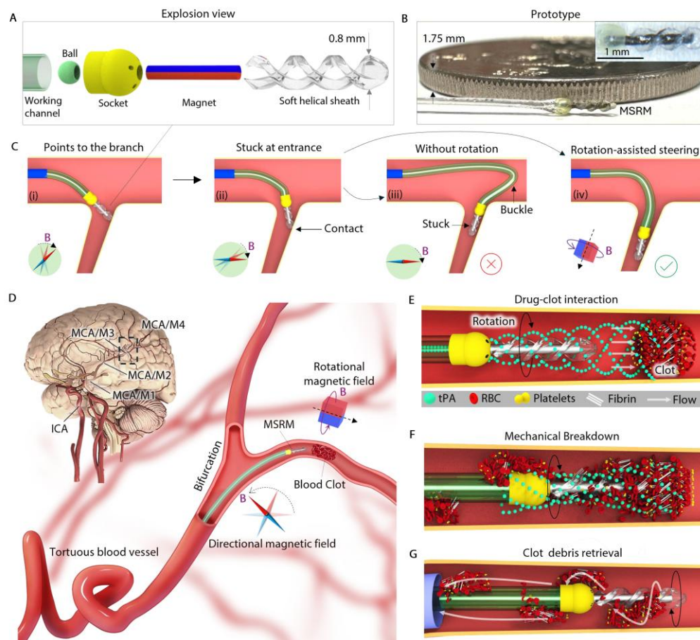
Fig.1 Conceptual diagram illustrating the design of the magnetic microcatheter system for endovascular treatments.
